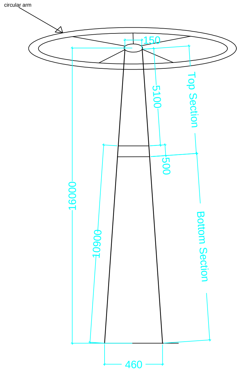
HIGH MAST POLE DIMENSIONS
