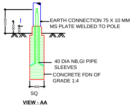
TYPICAL INSTILLATION OF STREET LIGHT POLE
