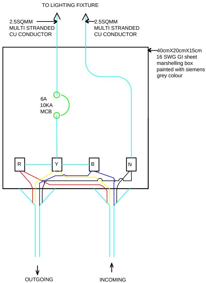
WIRING DIAGRAM OF MARSHALLING BOX
